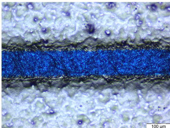
Screen printed, HF-compatible resist nitride passivation layer not etched
