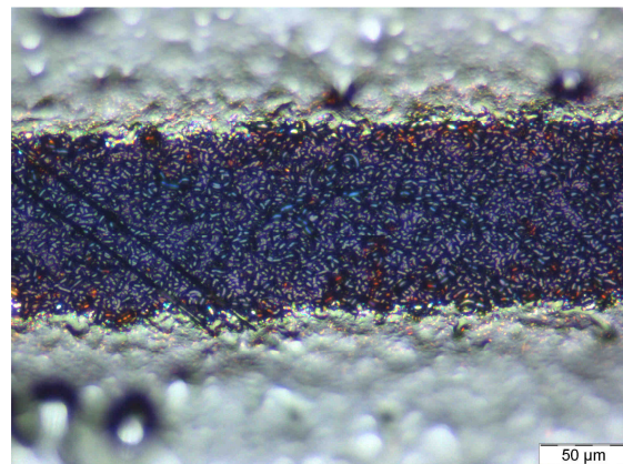
Screen printed, HF-compatible resist; porous silicon formed after HF-nitride-etch
