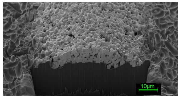
FIB cut of Ag paste finger, screen printed and fired; 50µm wide, 7.5µm thick
