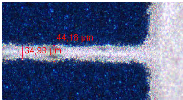
CCD picture of screen printed Ag paste finger for plating seed
